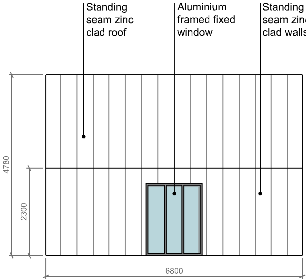
north elevation
