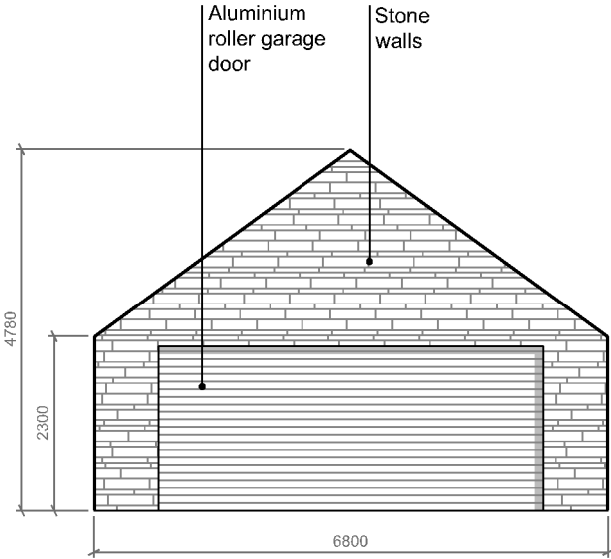
east elevation
