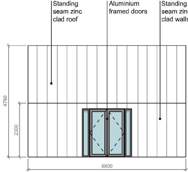
south elevation
