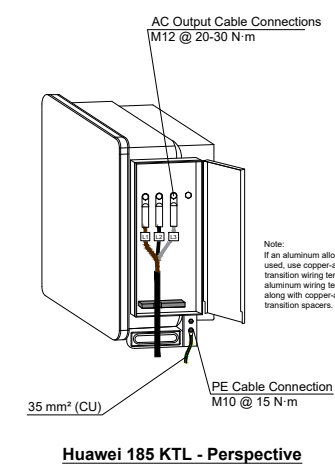
Huawei 185 KTL - Perspective
