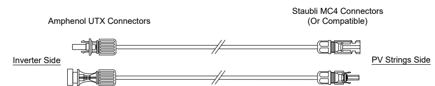
DC Cable Homeruns between Strings & Inverter
