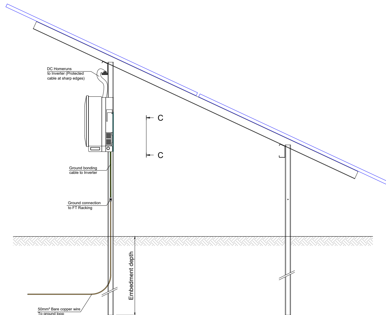
Inverter Mounting on Fixed Tilt Racking
