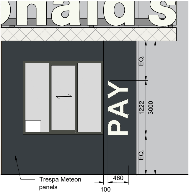
CASH BOOTH PAY SIGN NG100 & NG160
