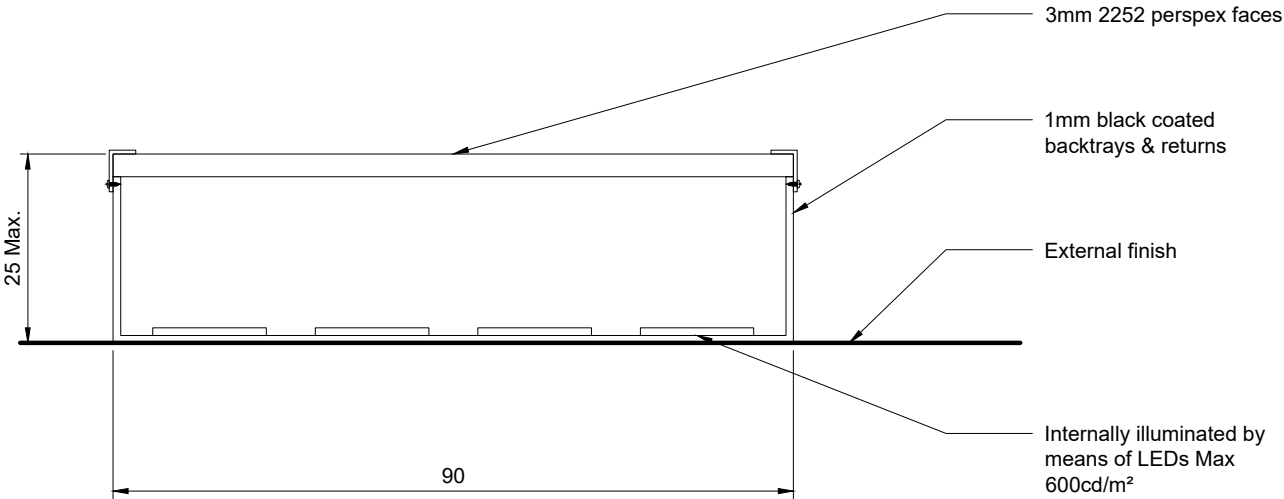
SECTION TYPICAL LETTER 1:1
