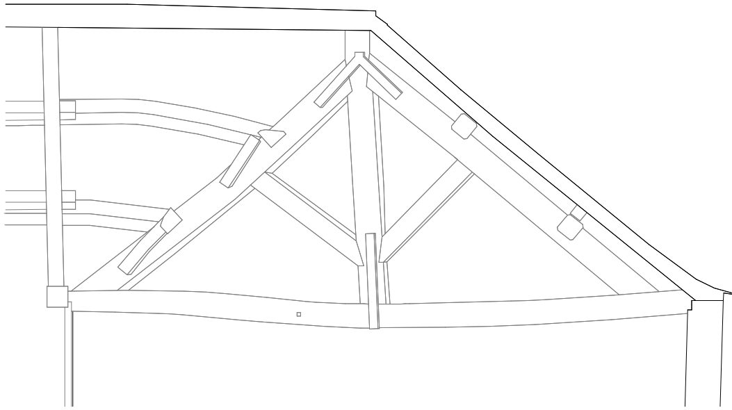
TYPICAL KING - POST TRUSS
