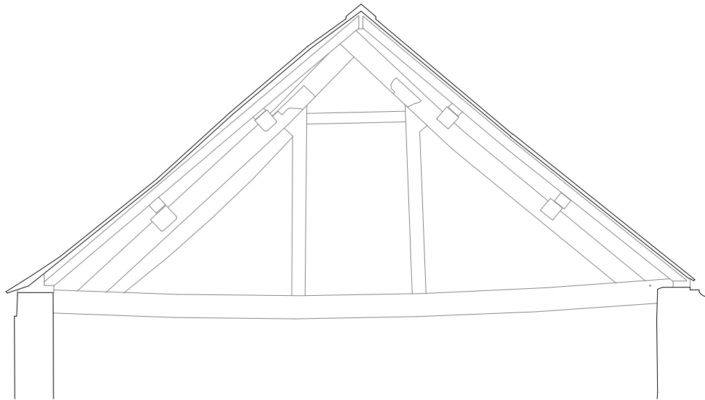
TYPICAL QUEEN - POST TRUSS
