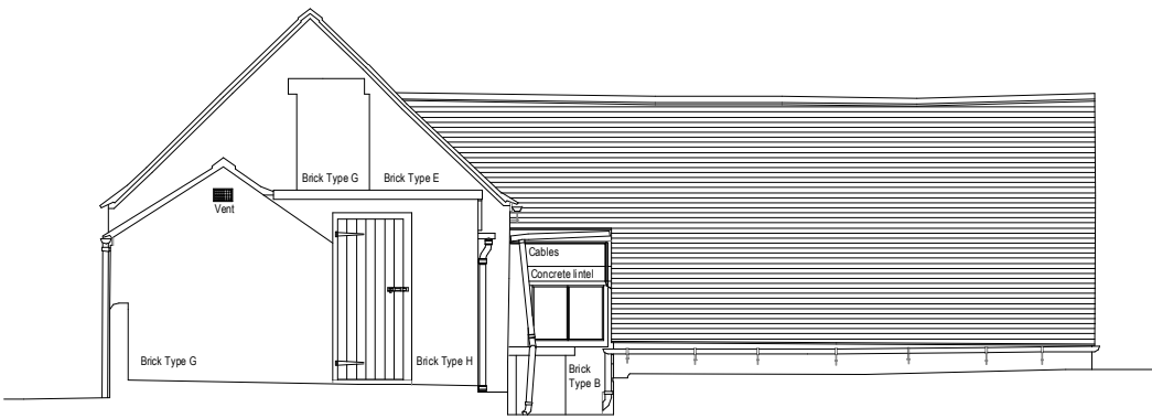
8 Shed North East Elevation 1 : 100
