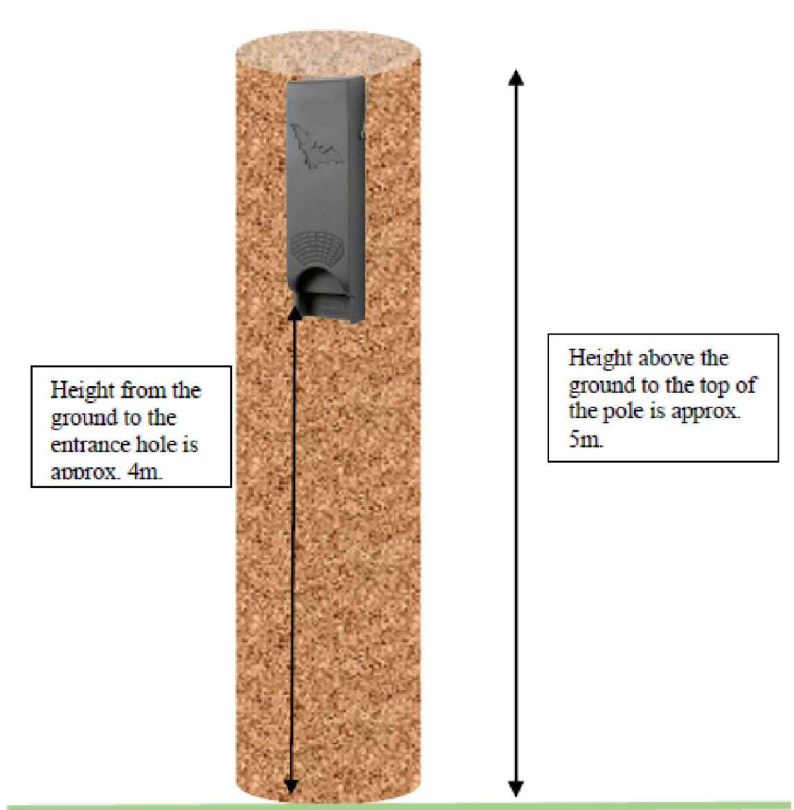
IMAGE OF TYPICAL POLE MOUNTED BAT BOX
