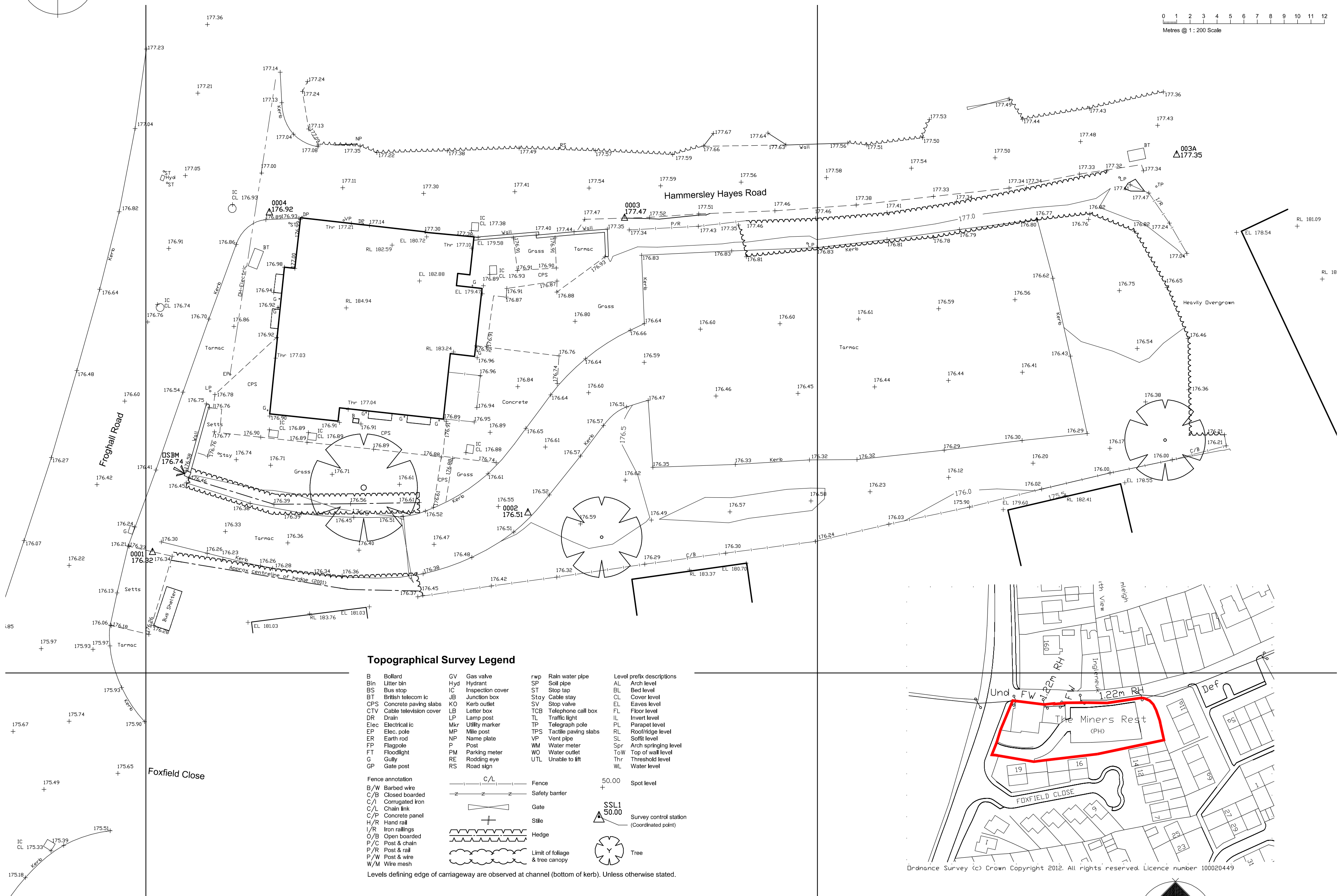
EXISTING SITE LAYOUT
