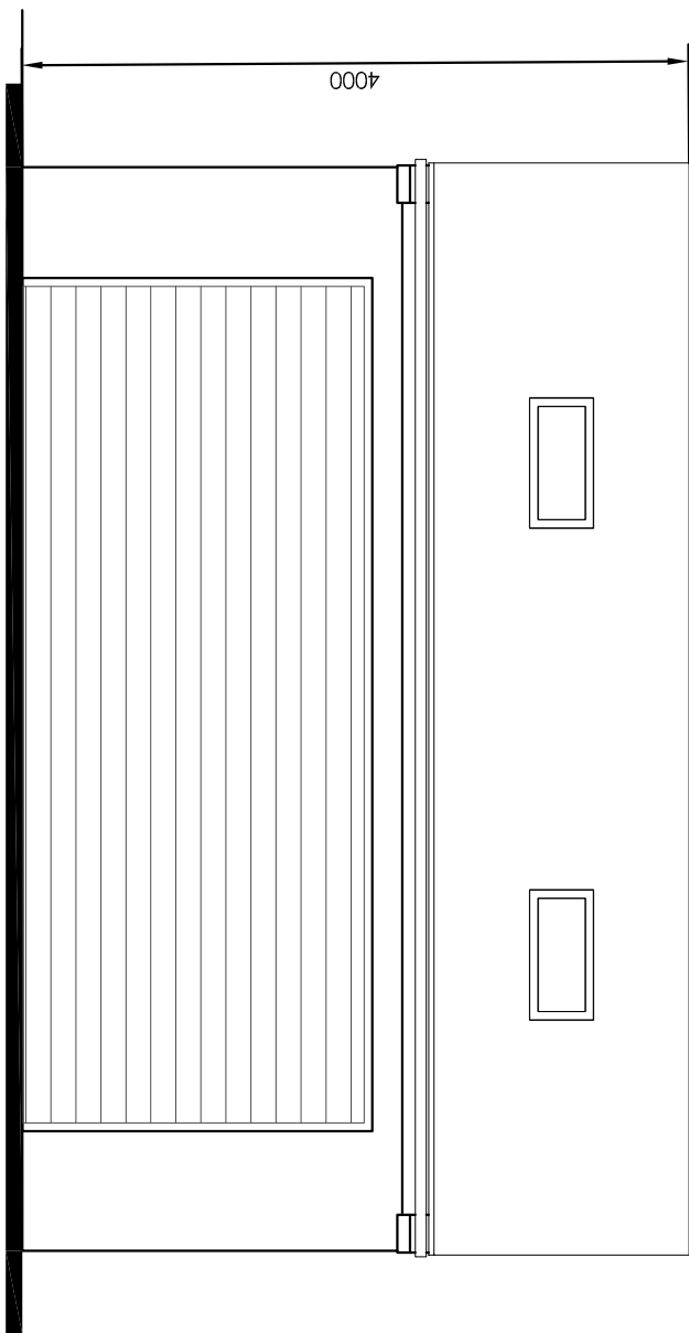
FRONT ELEVATION 1:50
