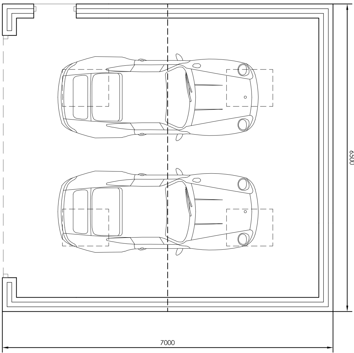
GARAGE FLOOR PLAN 1:50
