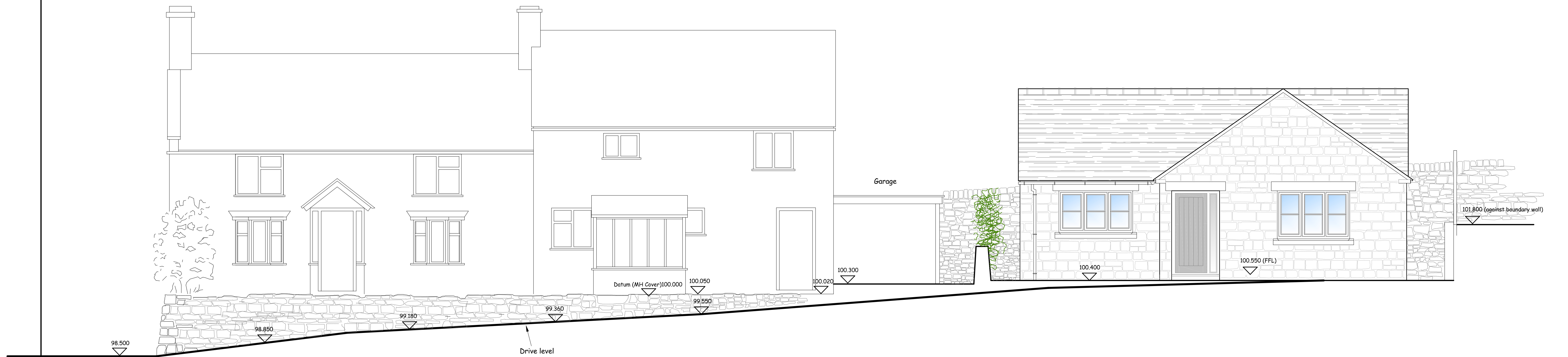
"STREET SCENE" WITH PROPOSED DWELLING
