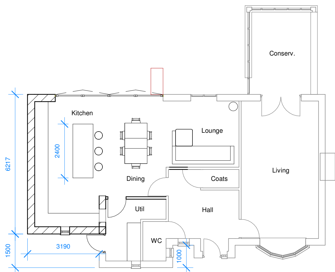
GFL Proposed 1 : 100
