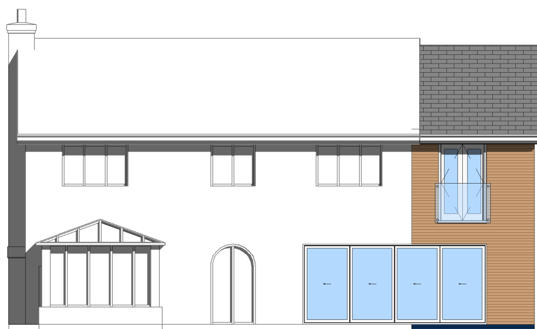
Rear Proposed 1 : 100
