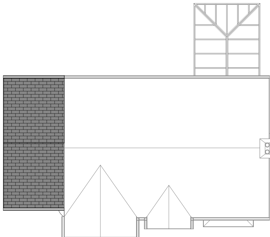
Roof Proposed 1 : 100
