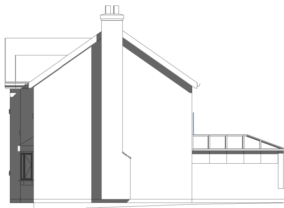
Side (NW) Proposed 1 : 100
