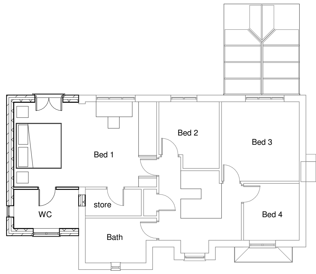
FFL Proposed 1 : 100
