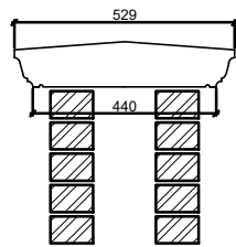
STONE COPING EXAMPLE
