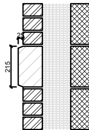
Length to match dimension of brick soldier course
