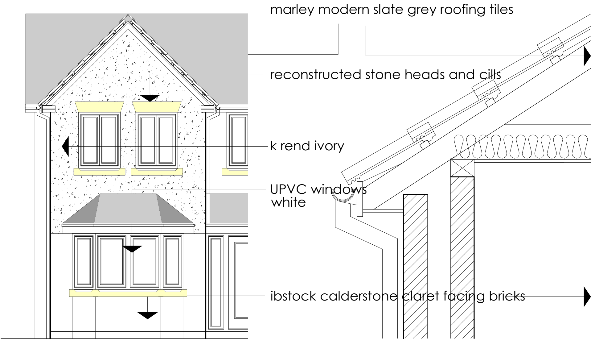
part elevation scale 1.50
