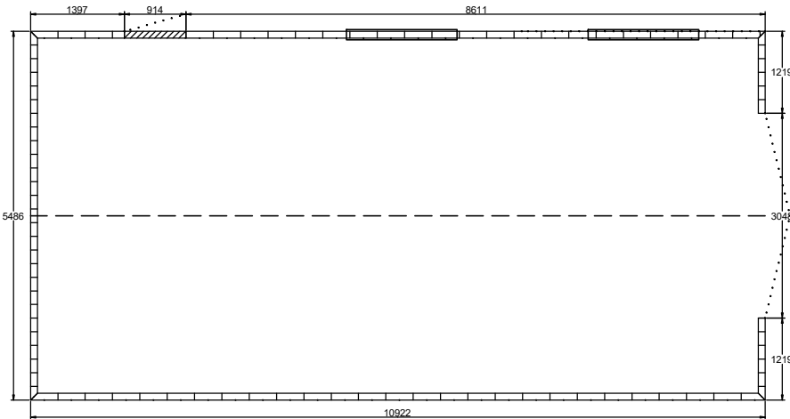
Base Plan
