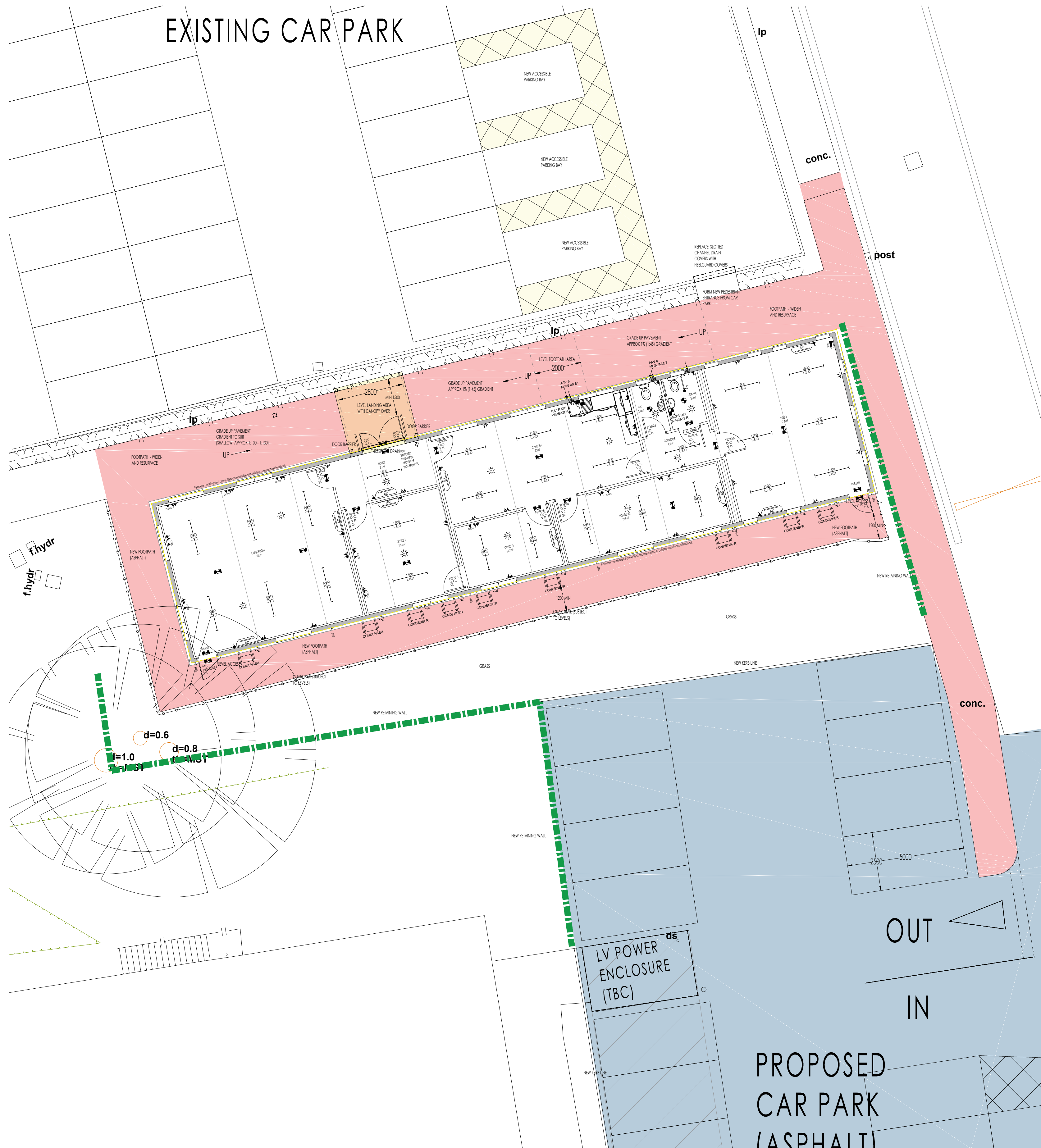
PROPOSED ETU LAYOUT PLAN SCALE 1:100@A1
