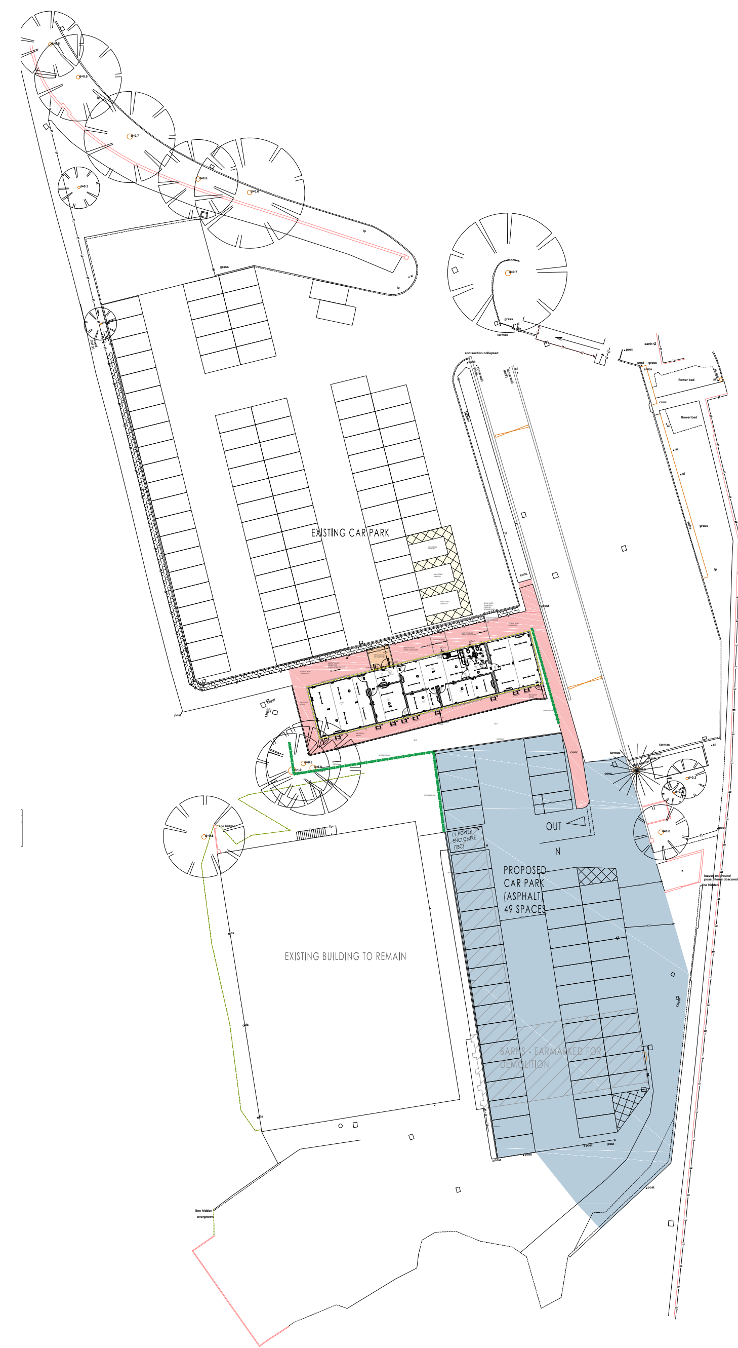
PROPOSED SITE LAYOUT PLAN SCALE 1:500 @ A1
