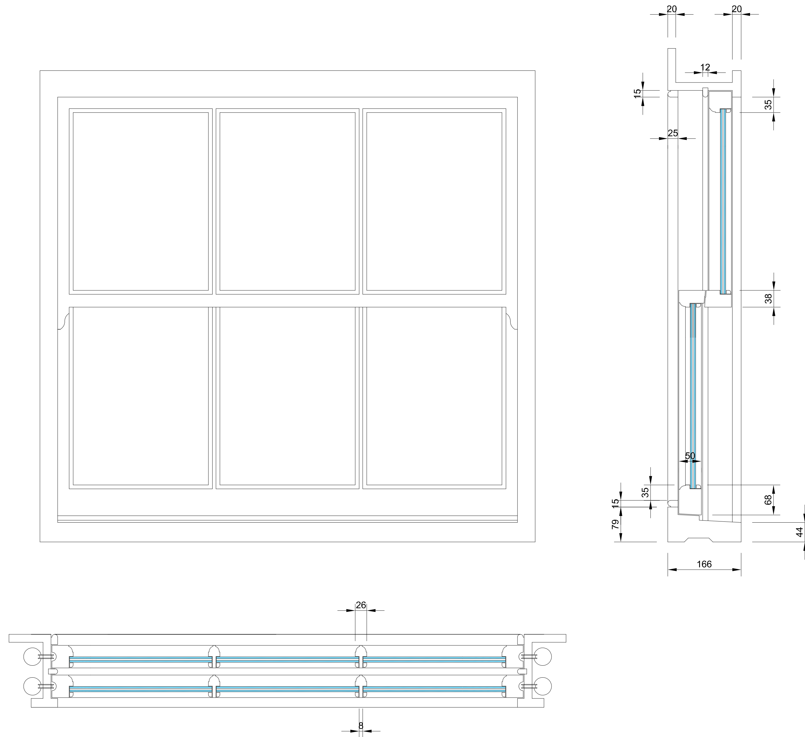
TRADIRIONAL, TIMBER, SLIDING SASH WINDOW DETAILS
