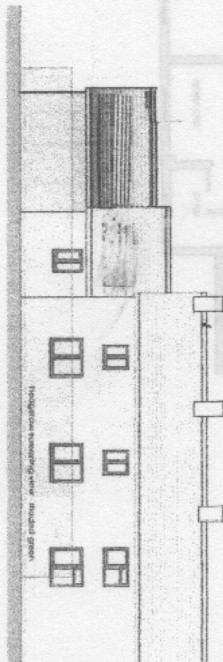
rear elevation - proposed
