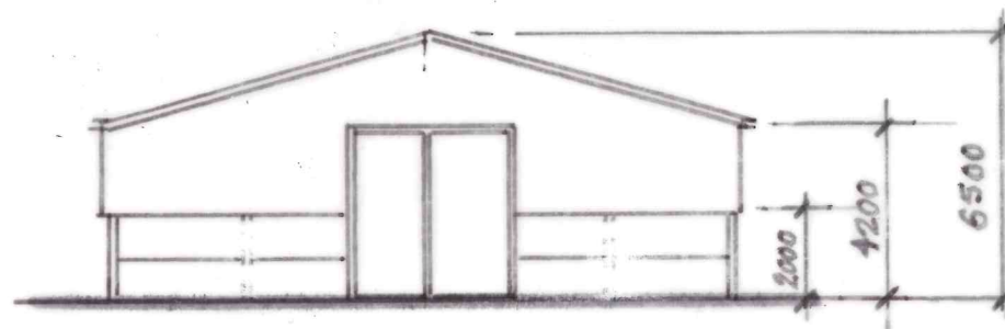
ELEVATION TO DRIVE.
