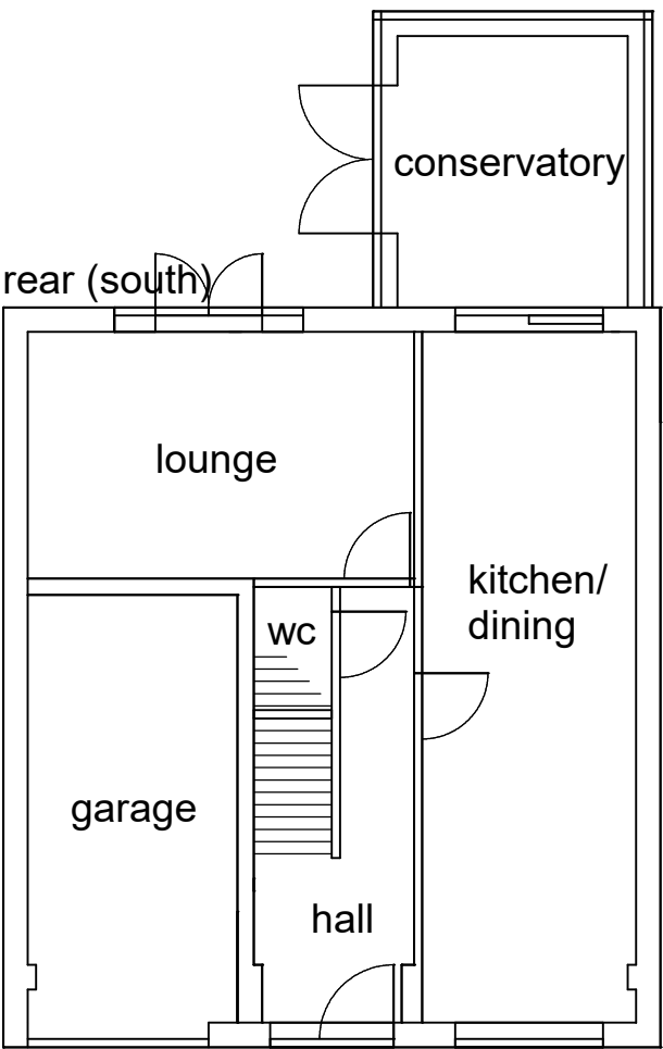
front (east) GROUND FLOOR LAYOUT
