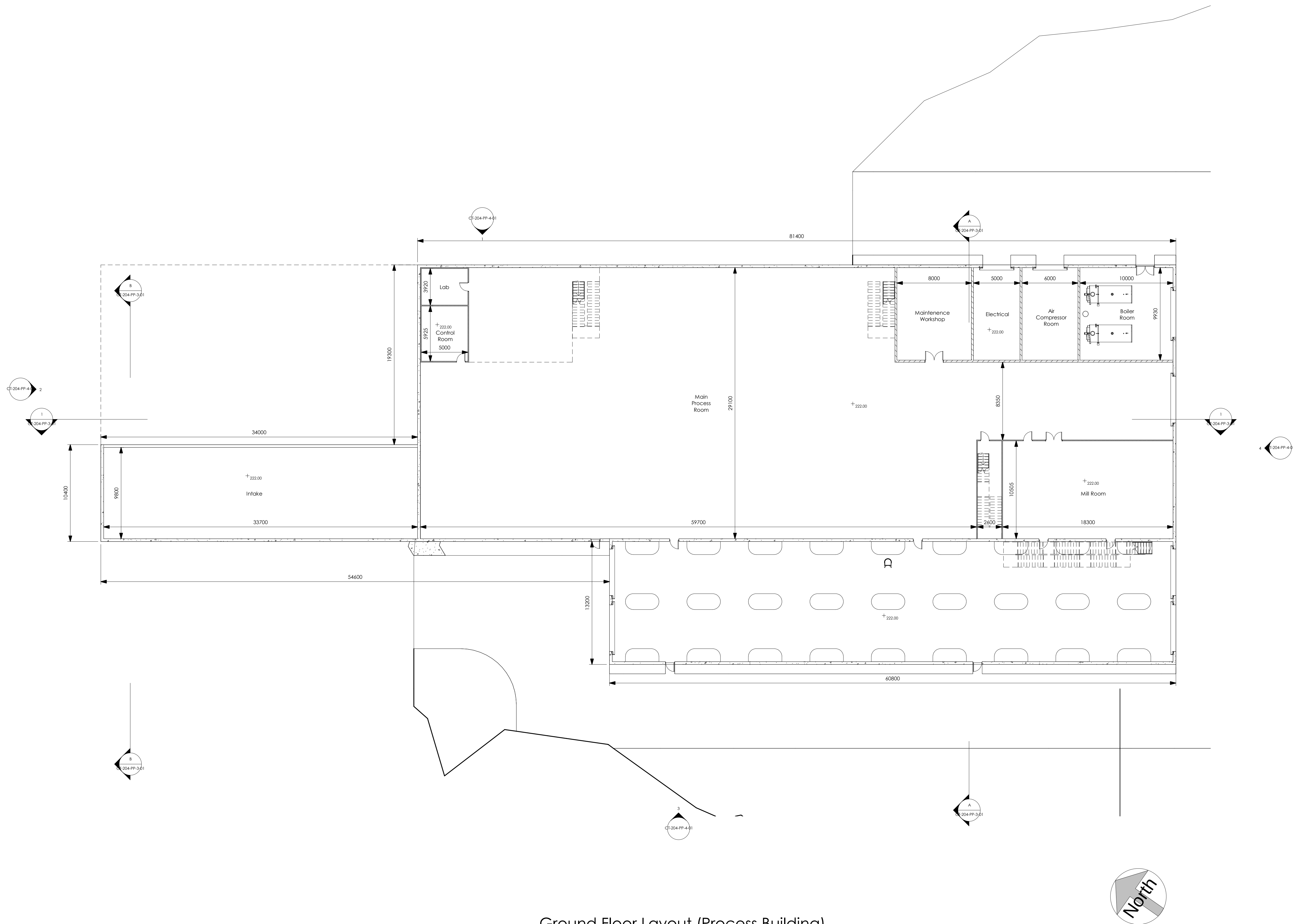
Ground Floor Layout (Process Building) 1 : 200
