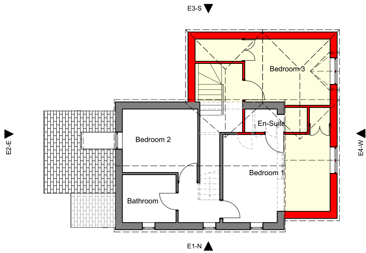
01-First Floor 1:100
