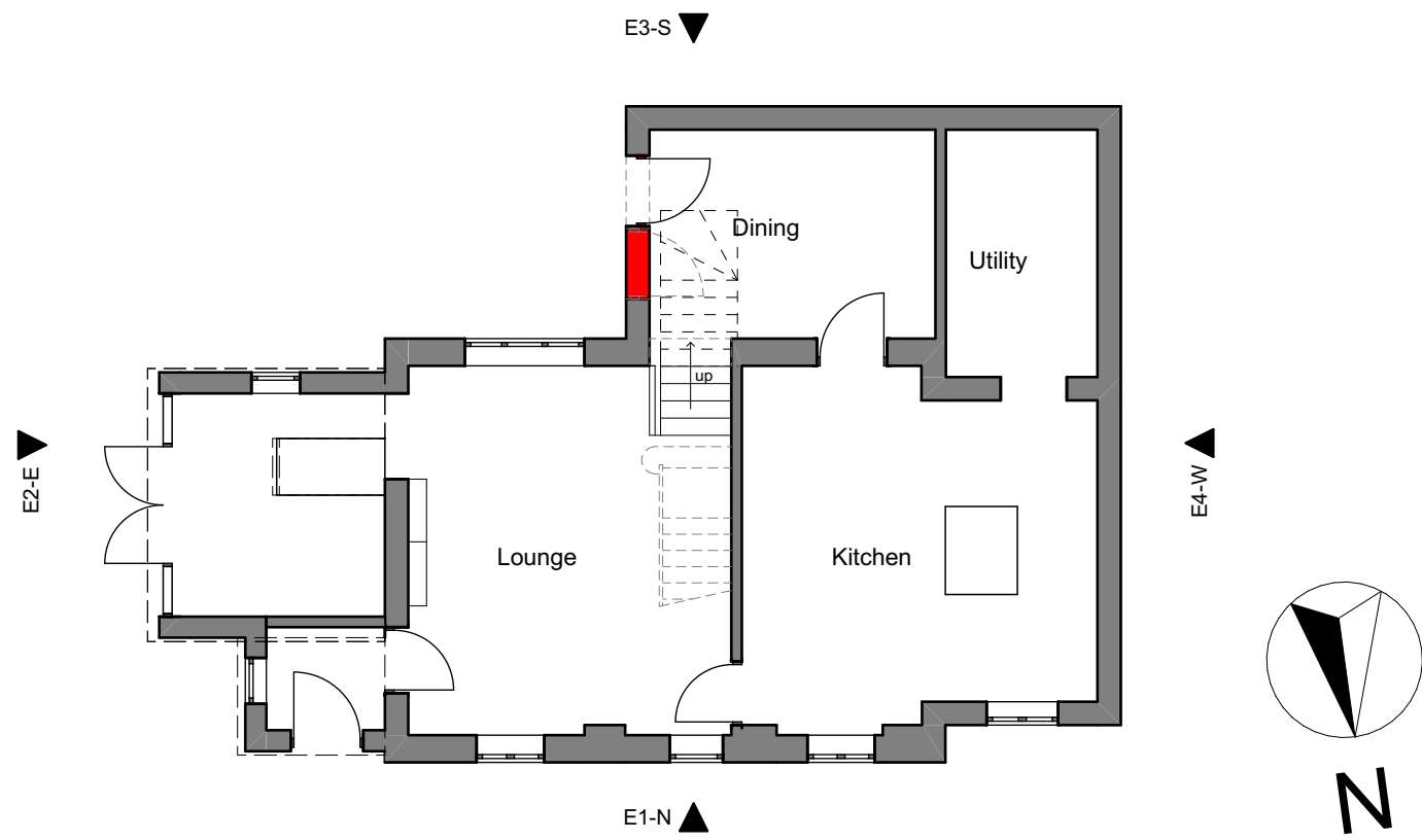
GF-Ground Floor 1:100
