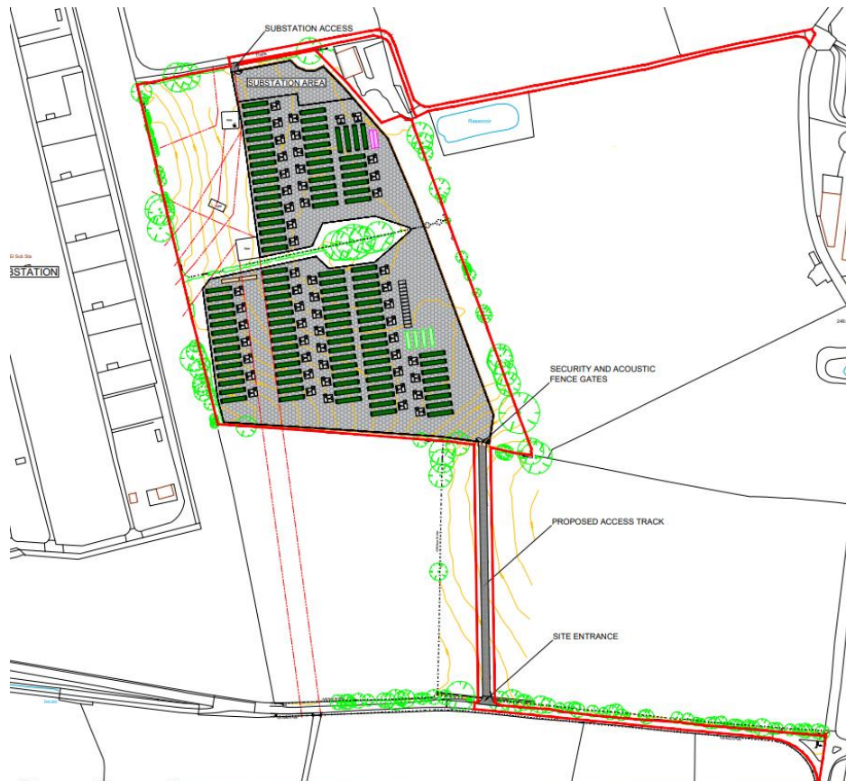
Figure 3.1 – Indicative Site Layout
