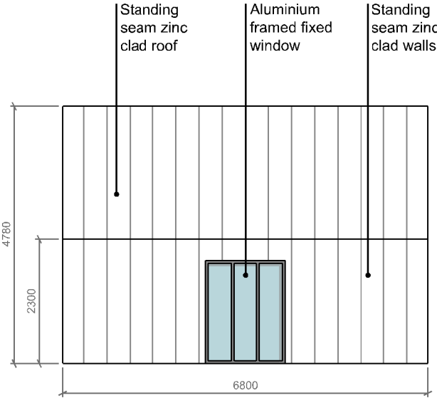
north elevation
