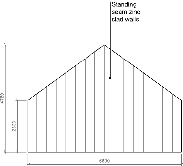
west elevation
