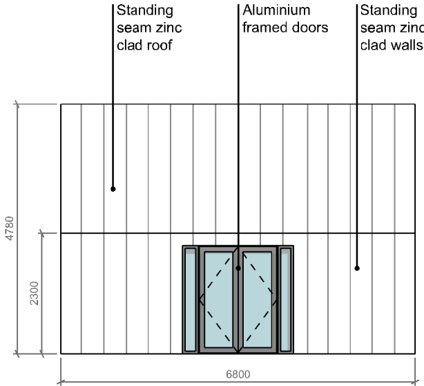
south elevation
