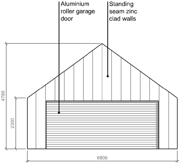
east elevation
