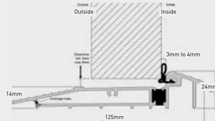
AM5EX (Mobility Threshold) (open out)
