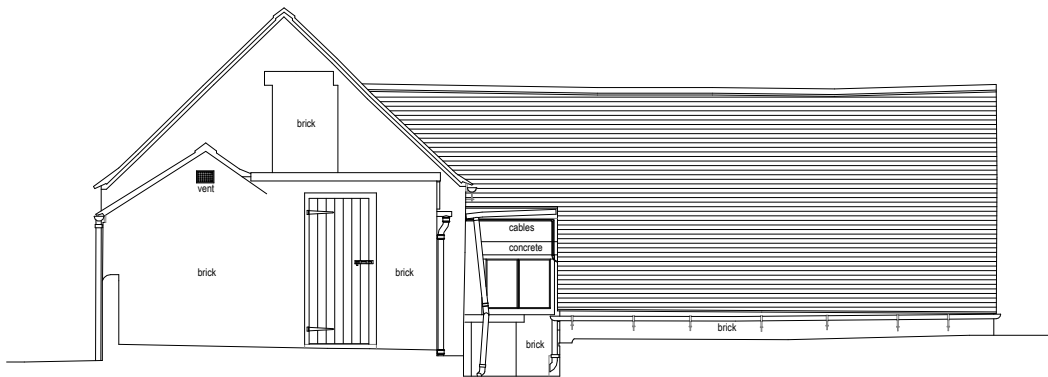
8 Shed North East Elevation 1 : 100
