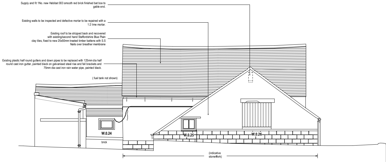
8 Shed North West Elevation Proposed 1 : 100
