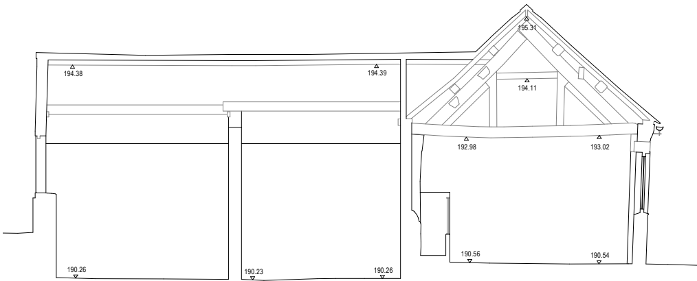
8 Shed Section A-A Proposed 1 : 100
