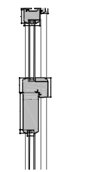
win .01 Detail: B
