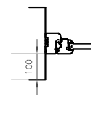
win .03 Detail: B
