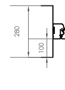
win .04 Detail: A
