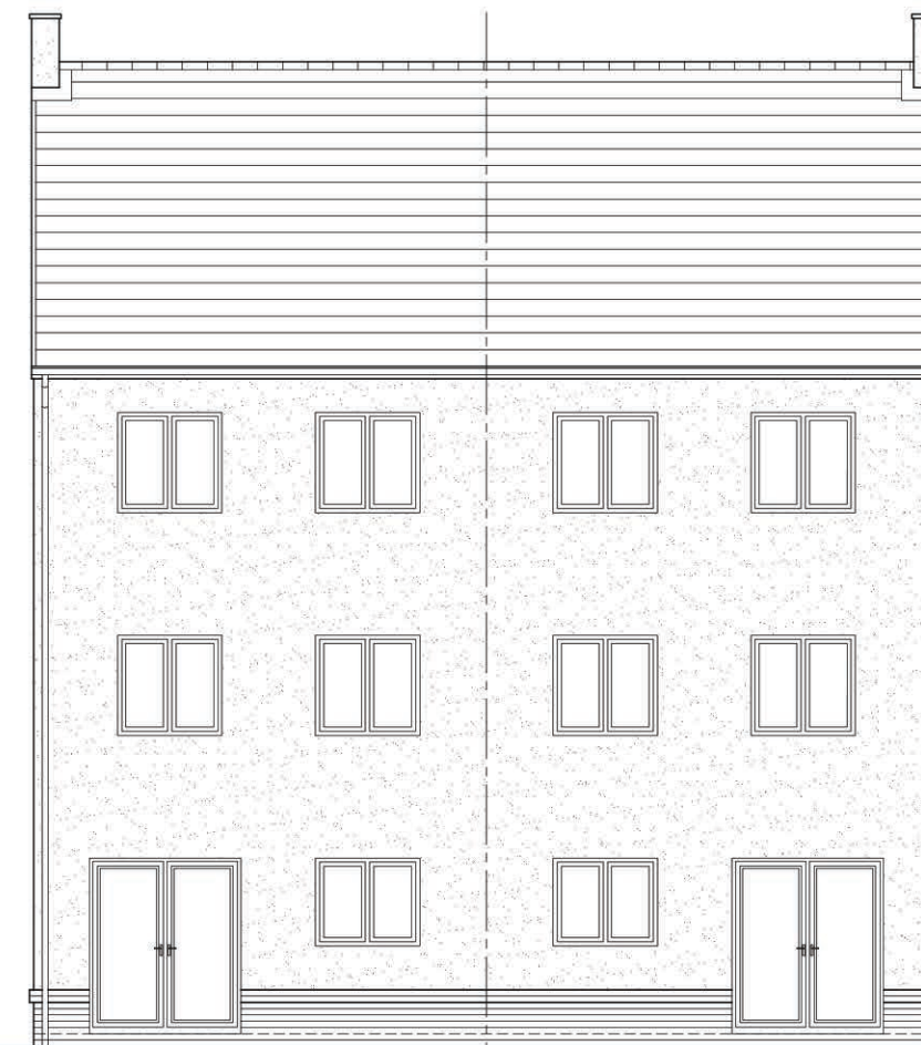
Rear Elevation
