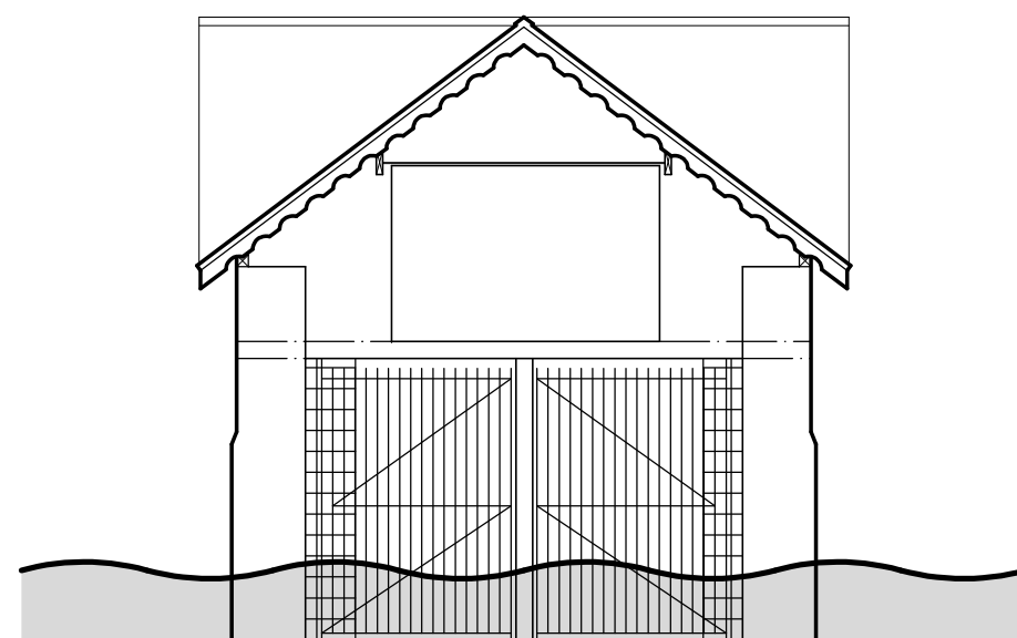
North-East Elevation
