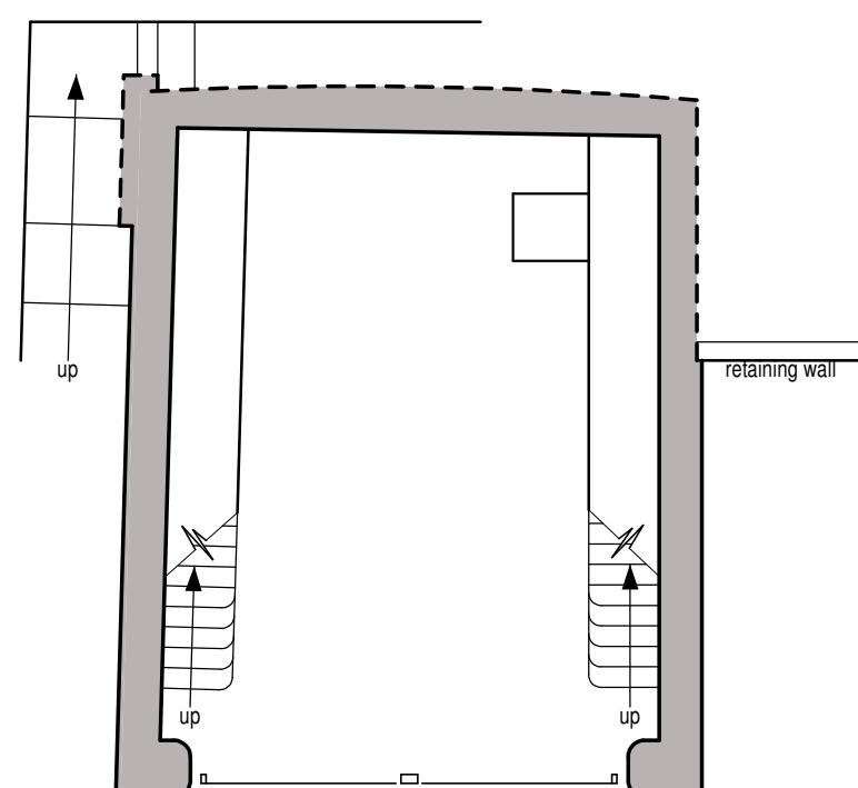
Docking Level
