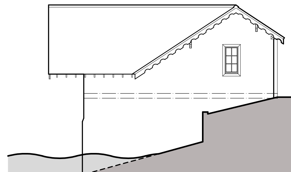
North-West Elevation
