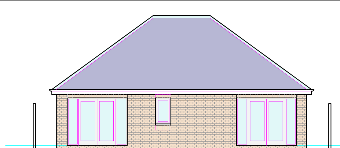
REAR ELEVATION
