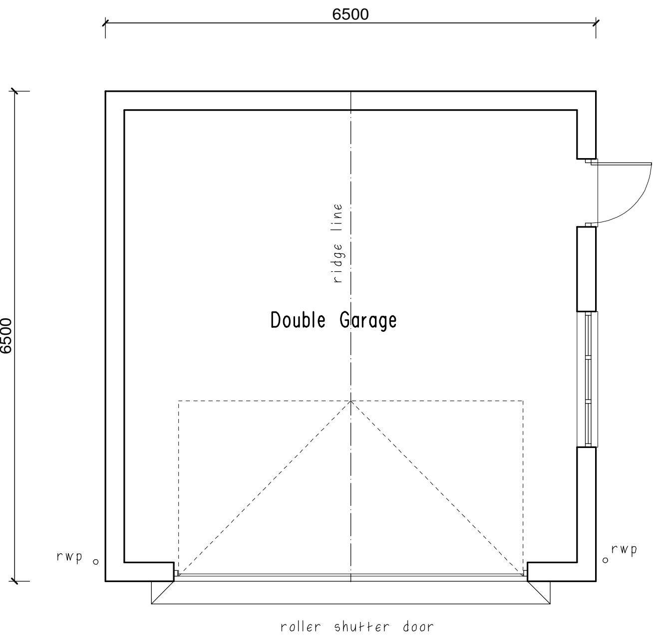
Floor Plan
