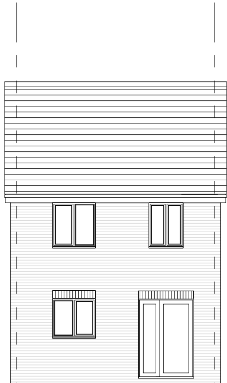
Rear Elevation
