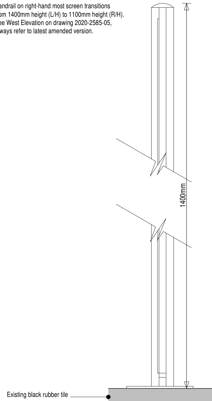
Cross Section through Privacy Screen
