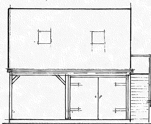
EAST ELEVATION
