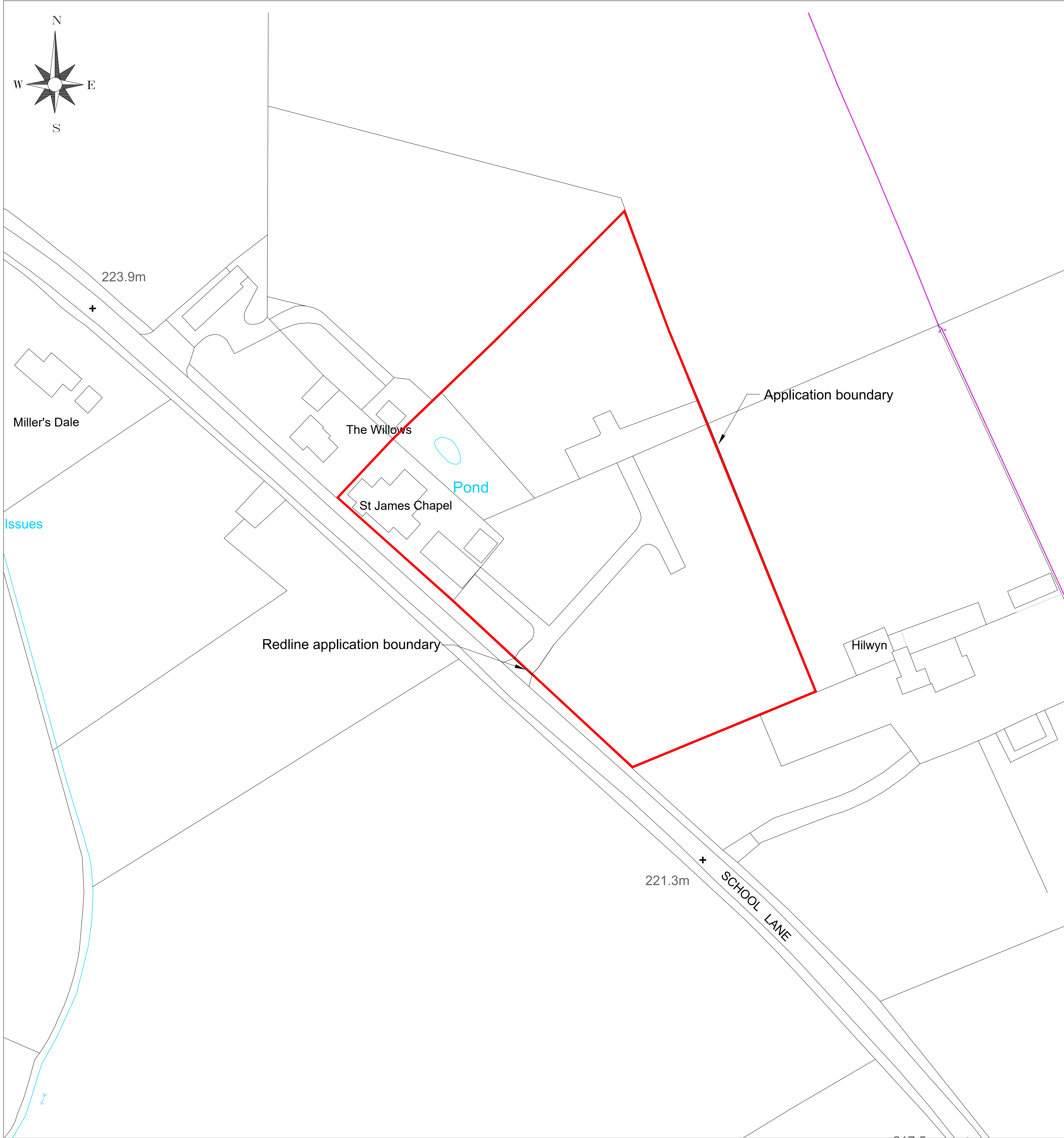
LOCATION PLAN 1:1250
