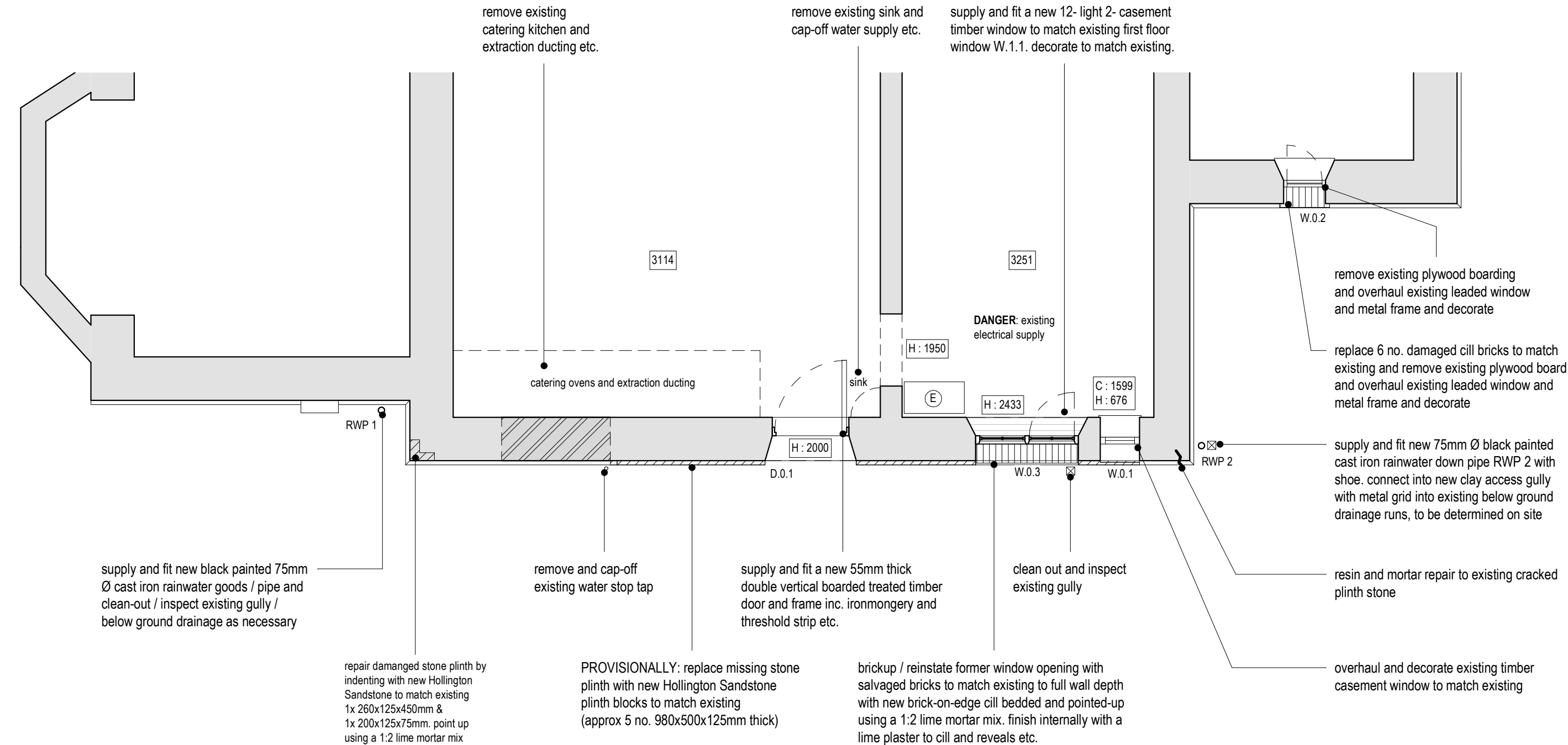
Ground Floor (Part Plan)
