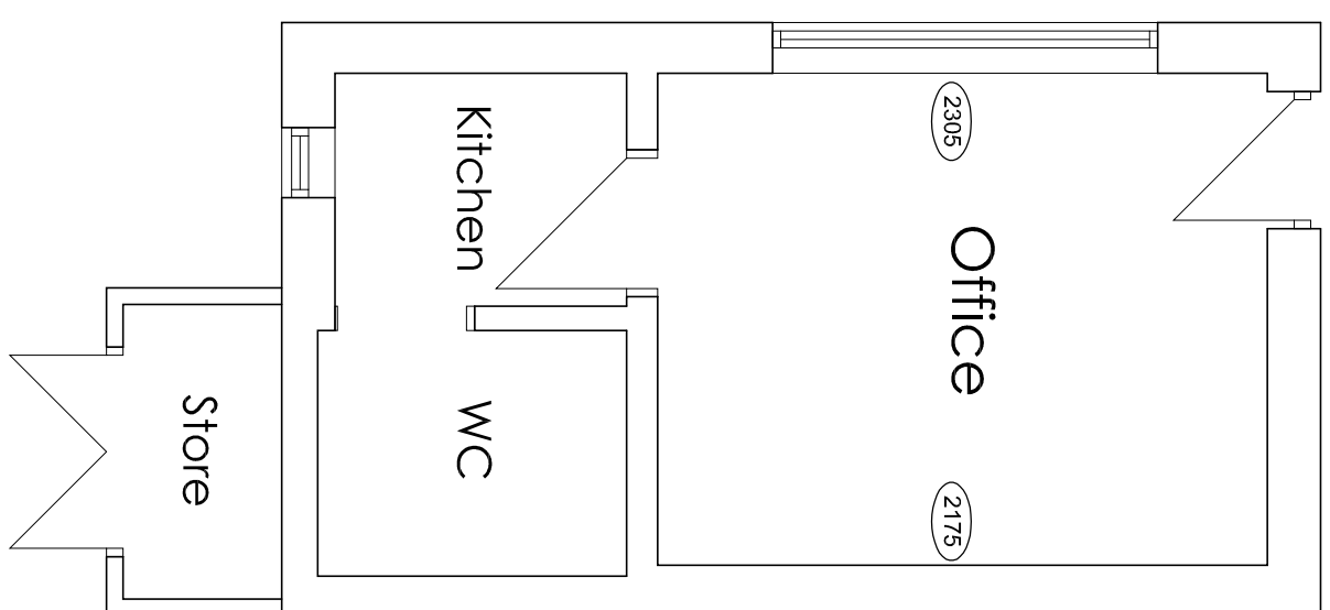
FLOOR PLAN 1:50
