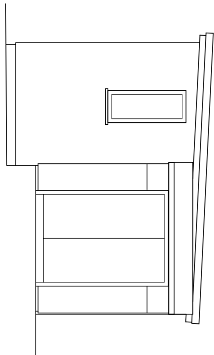
REAR ELEVATION 1:50
