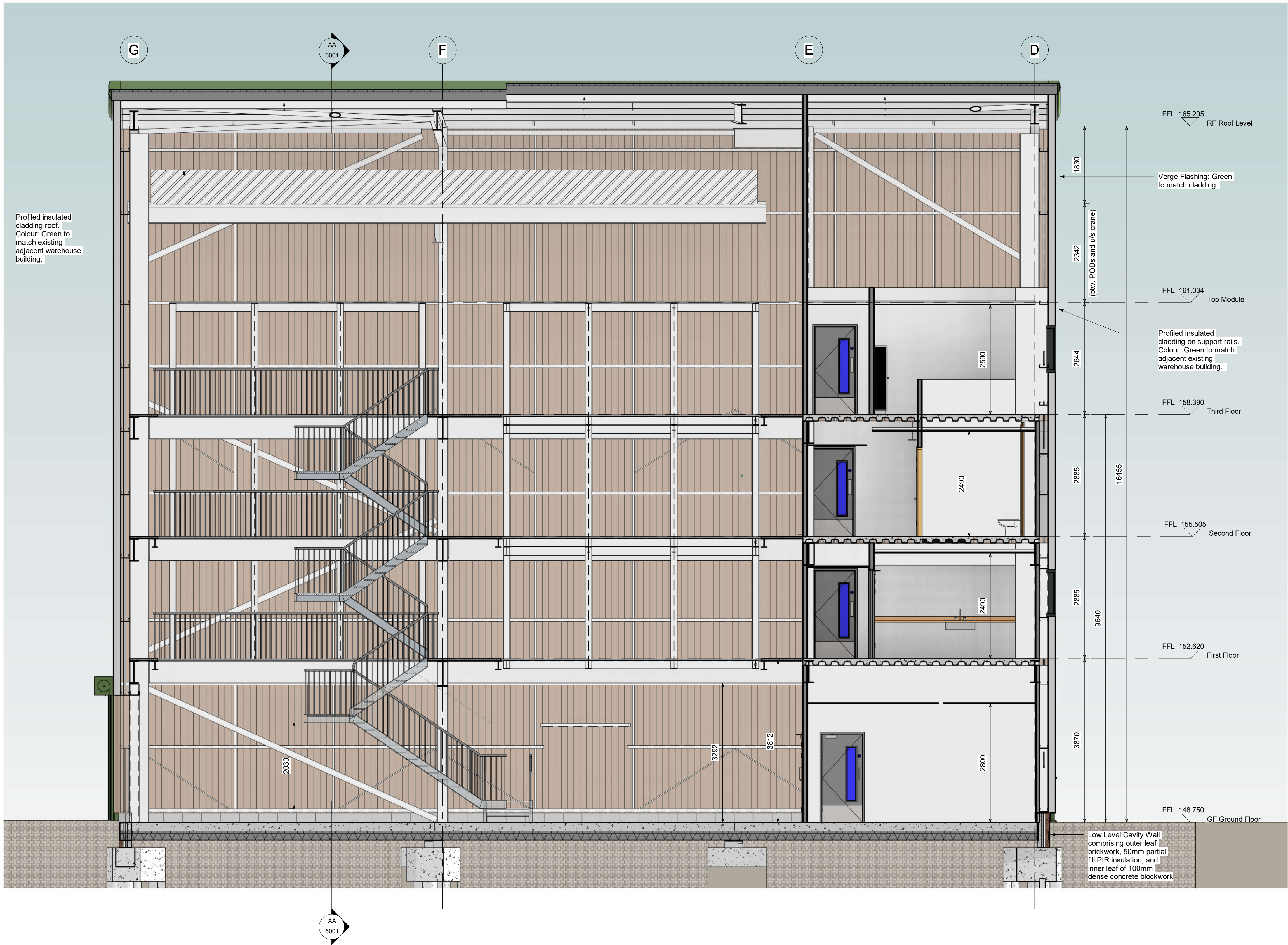
BB Building Section 2 1 : 50
