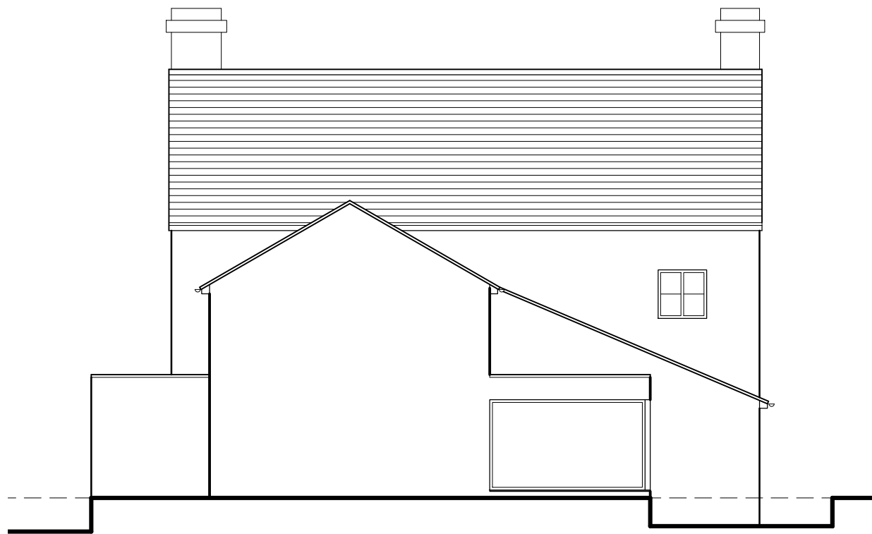
Rear Elevation (North-East)
