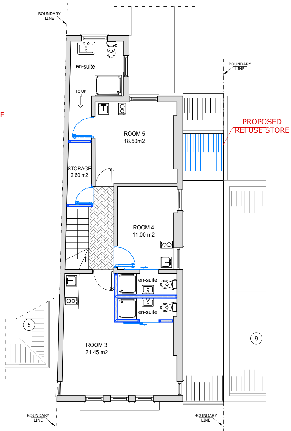
PROPOSED SECOND FLOOR PLAN SCALE: 1/100 @A3
