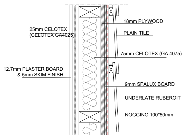
DETAIL 6 TYPICAL DETAIL OF EXTERNAL STUD WALL CONSTRUCTION (ISOMETRIC)
