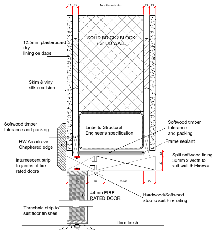
DETAIL 4 TYPICAL DOOR JAMB DETAIL(head plan)
