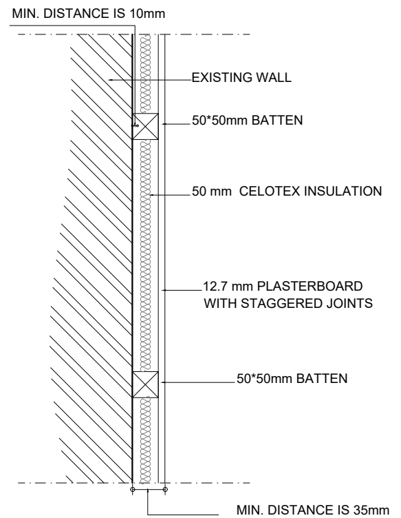
DETAIL 5 EXISTING EXTERNAL WALL TREATMENT (FOR ENERGY SAVING AND NOISE)
