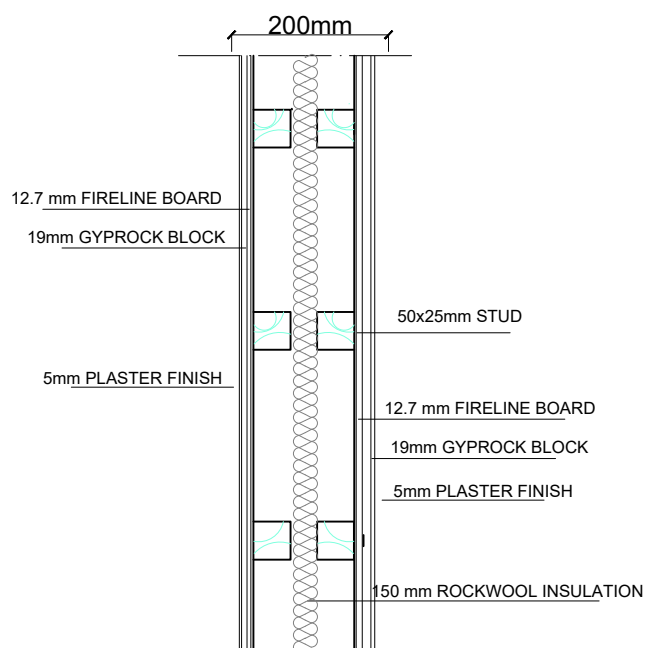
DETAIL 1 FIRE&SOUND INSULATION DETAIL TO PARTITION WALL BETWEEN THE ACCOMMODATION AND THE COMMON STAIRCASE & INNER BEDROOMS
