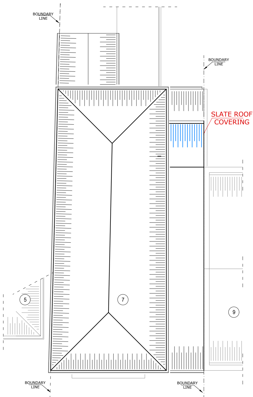
PROPOSED ROOF PLAN SCALE: 1/100 @A3
