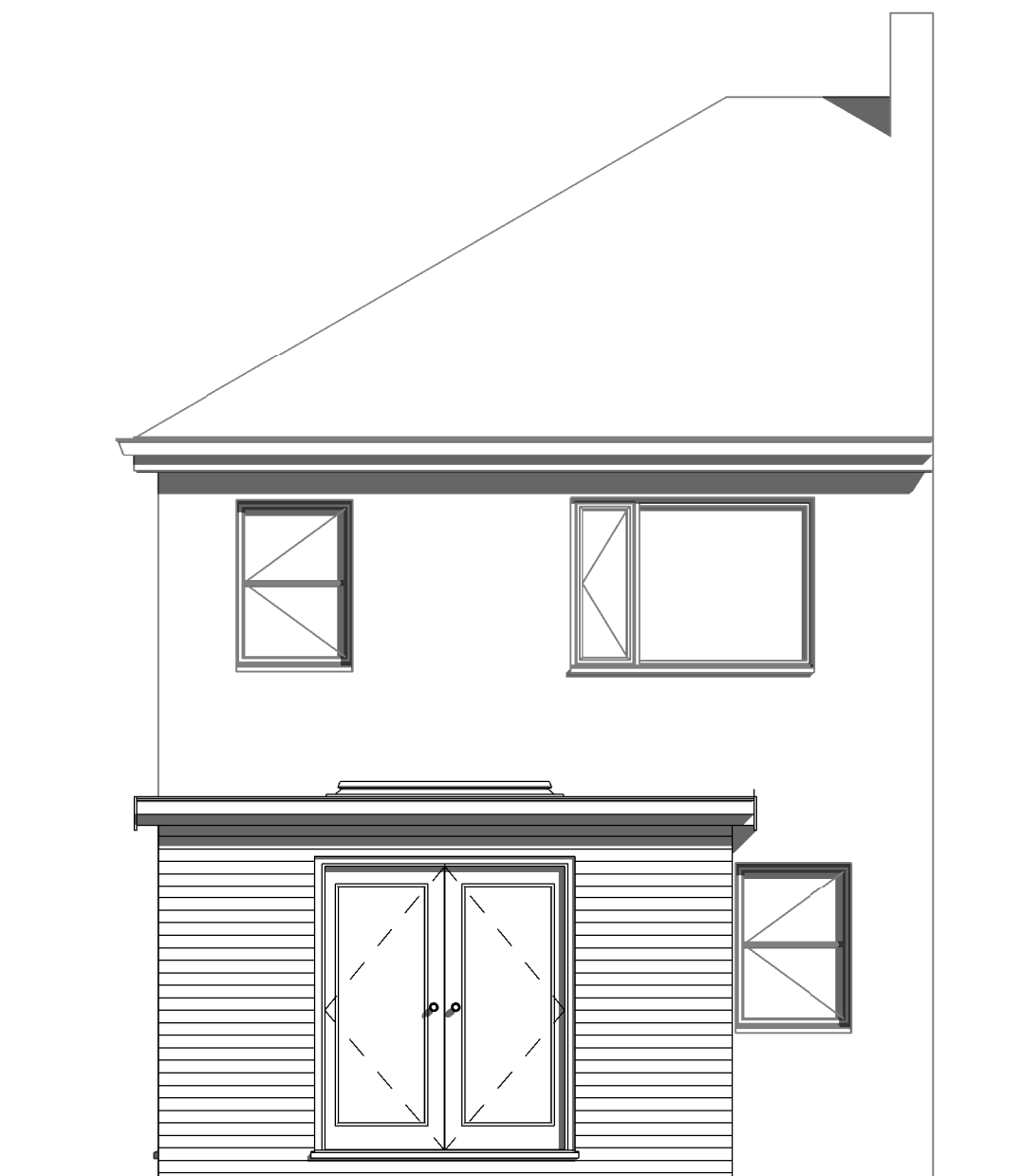
5 Rear Proposed 1 : 50
