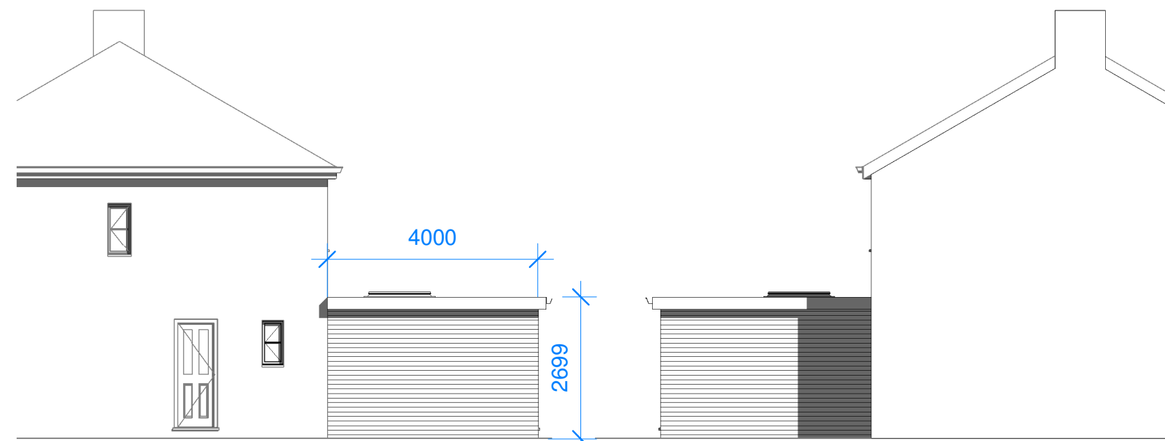
7 Side Proposed 1 : 100
