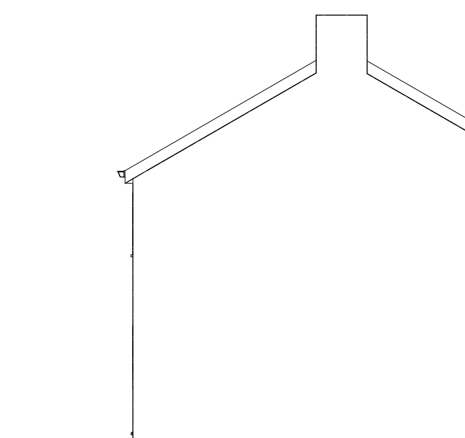
10 Party Existing 1 : 100
