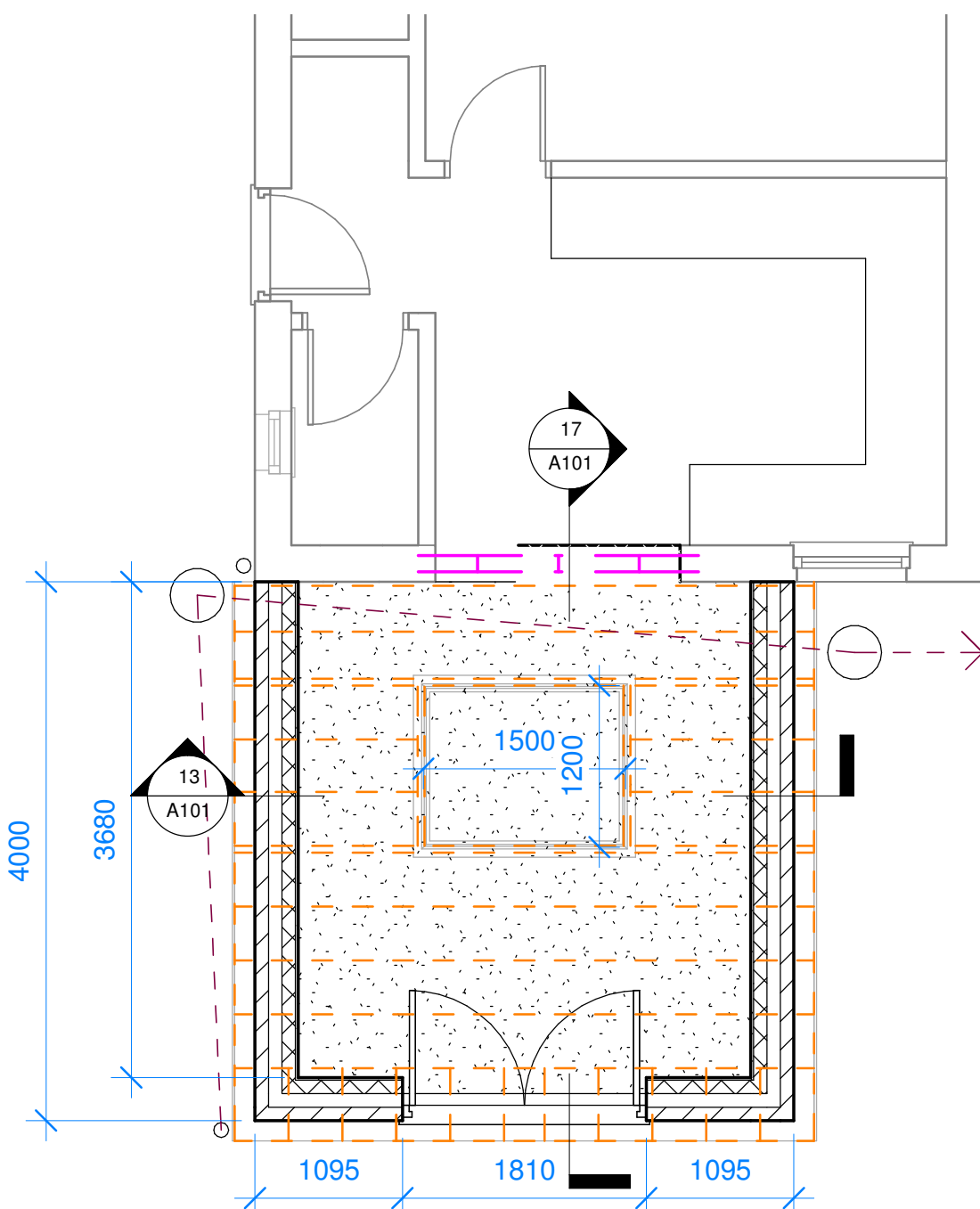
4 GFL Proposed 1 : 50
