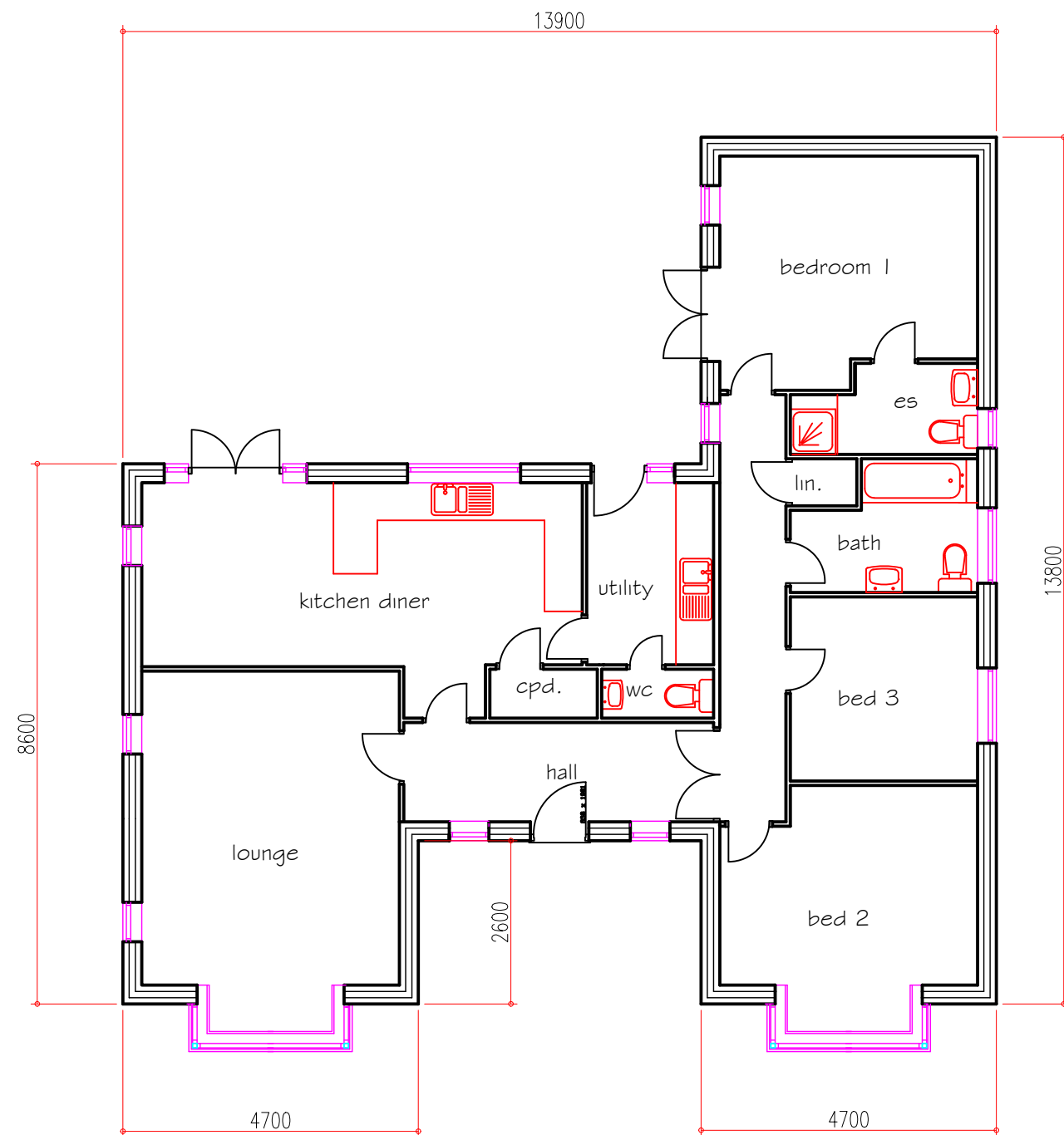
Floor Plan
