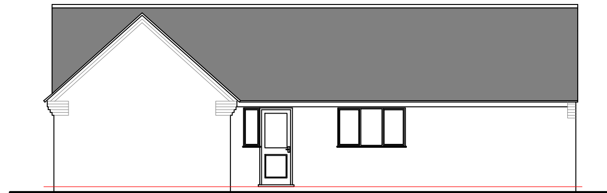
Rear (SW) Elevation
