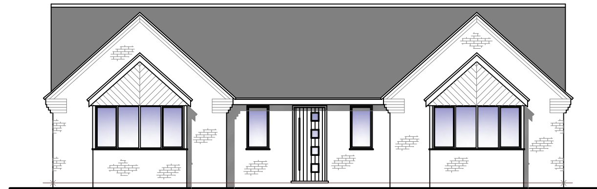
Front (NE) Elevation
