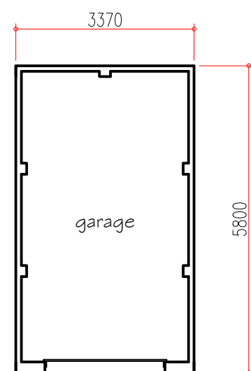
Garage Plan
