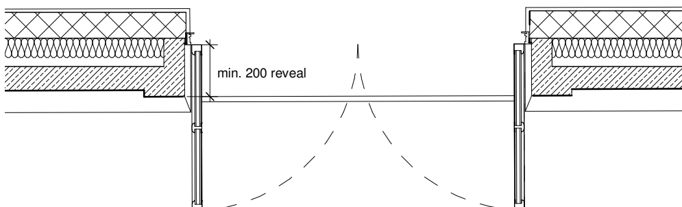
typical door plan detail
