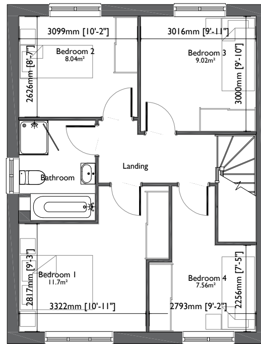
First Floor Plan Scale 1:200
