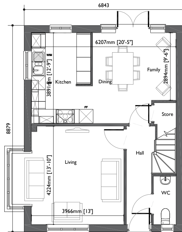
Ground Floor Plan Scale 1:200
