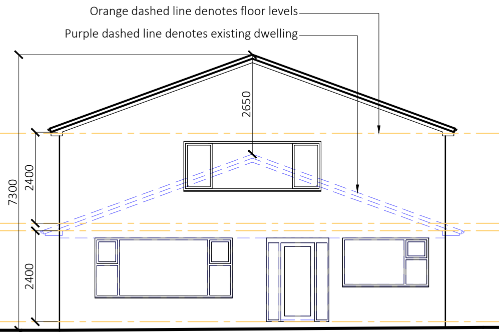
Front Elevation (South West)
