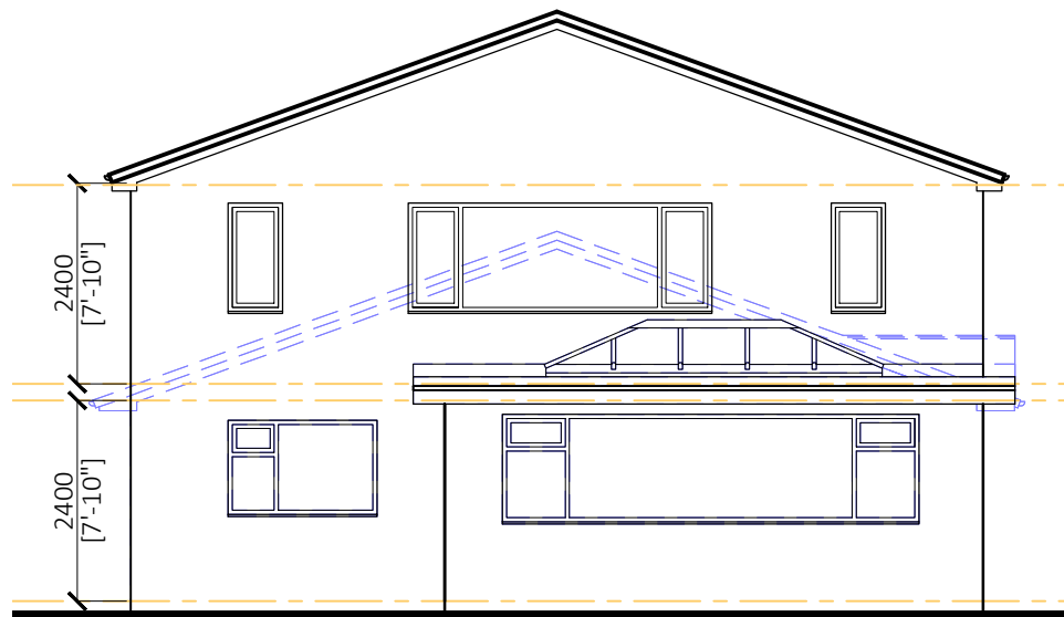
Rear Elevation (North East)
