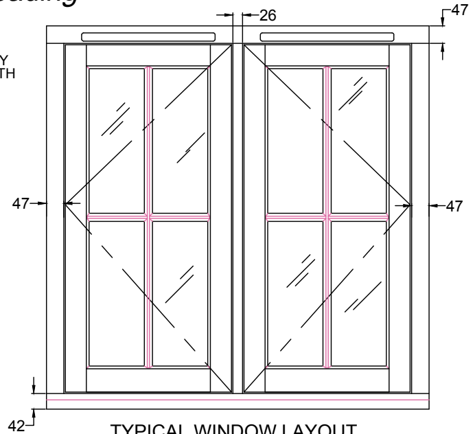
TYPICAL WINDOW LAYOUT
