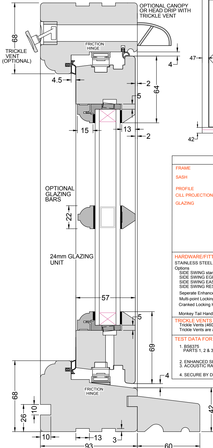
TYPICAL WINDOW LAYOUT
