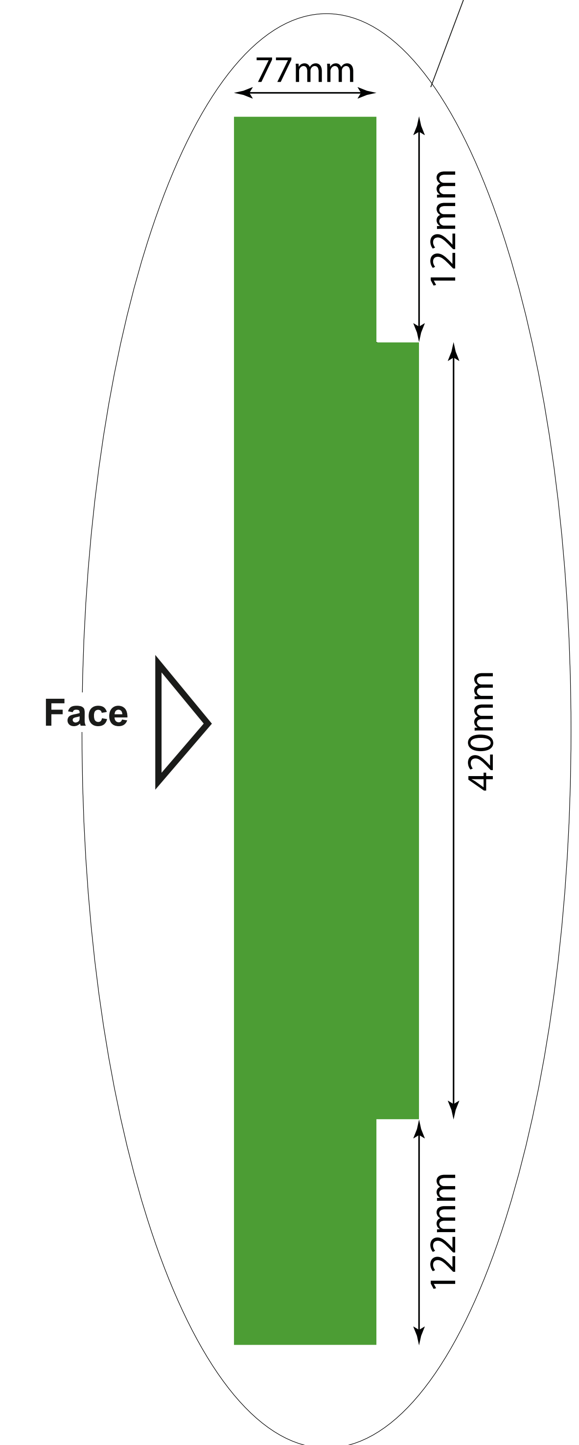
Panel Edge Profile Scale 1:2
