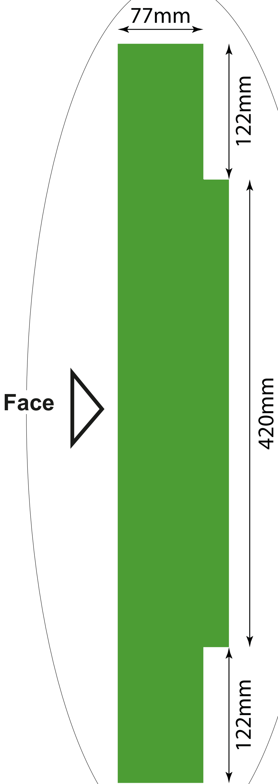
Panel Edge Profile Scale 1:2
